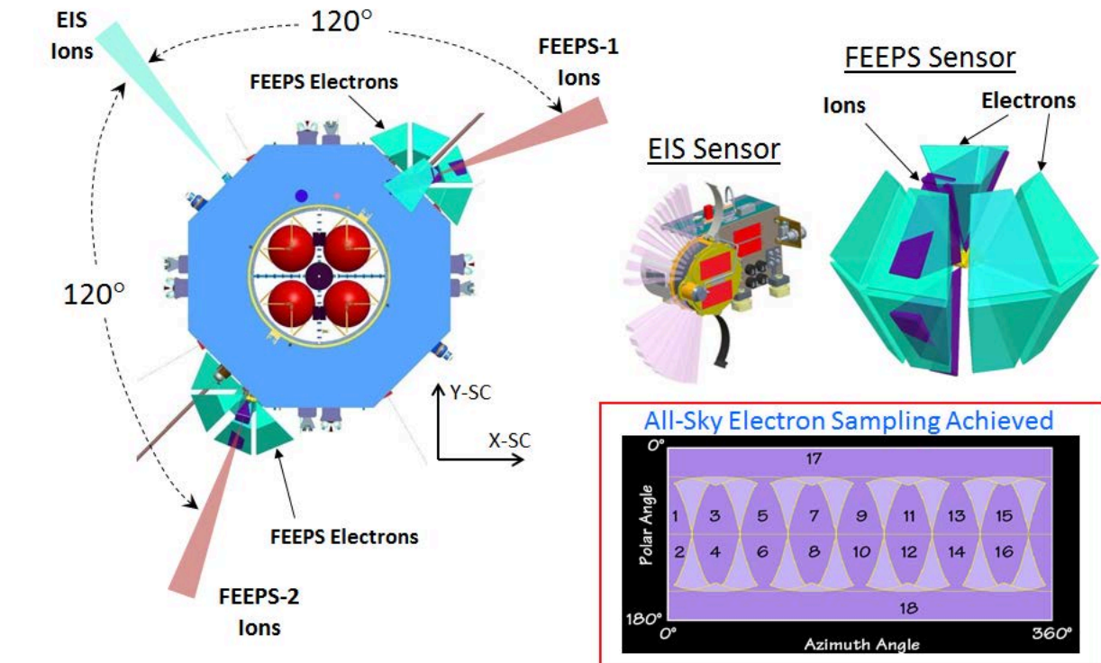
Figure 6-2 The EPD fields-of-view are Configured to Provide Maximum Sky Coverage of Energetic Particles. [The two FEEPS sensors provide nearly simultaneous full-sky electron coverage, whereas the two FEEPS sensors complement the EIS fan-shaped FOV to provide ion coverage in approximately 1/3 of a spin.] (from Mauk et al. [2016])
