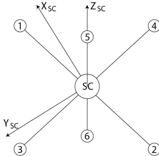
Figure 11-1 Schematic of SDP and ADP Probes
